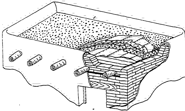
Figure 85. The cutaway section of this bunker fill roof shows the layered structure of the roof. From the top down, the components are gravel and asphalt, building paper, earth fill, building paper, wood sheathing and supporting beams (vigas).
