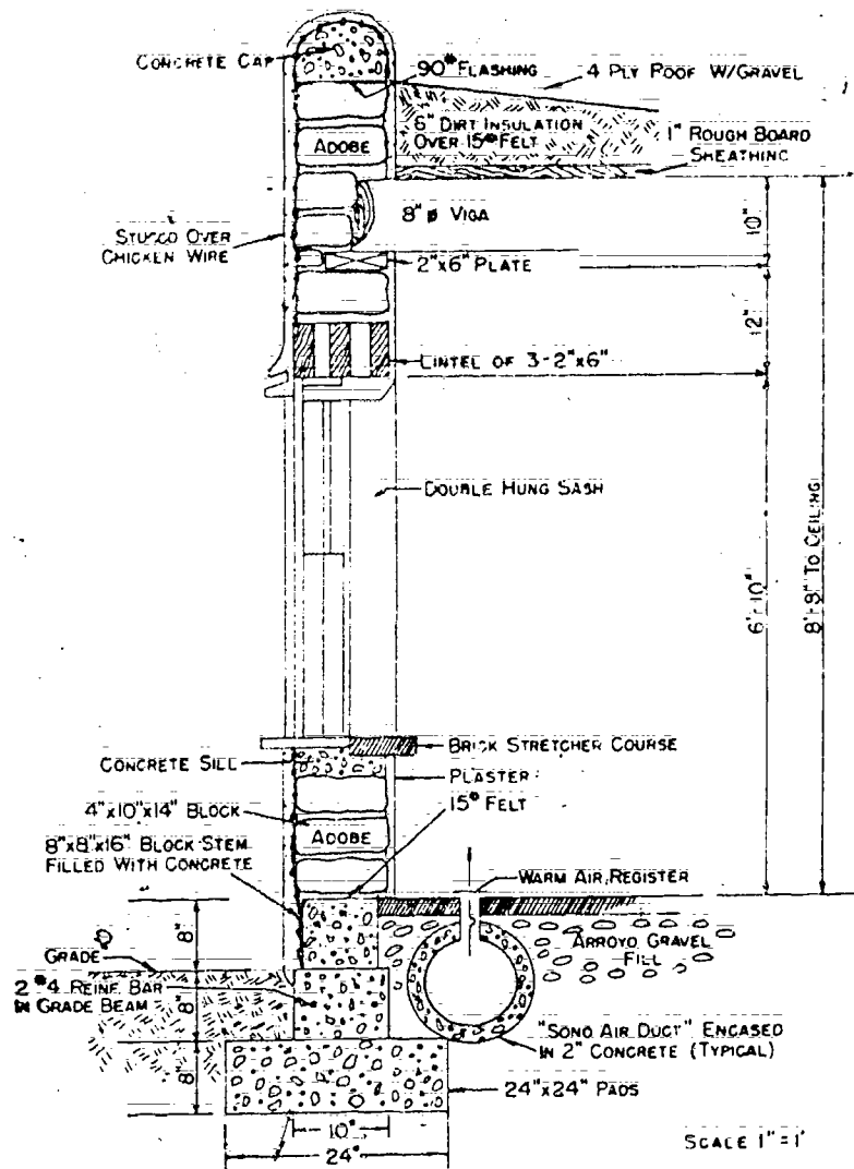
Figure 64. A builder in Albuquerque, N. M., uses this wall section for adobe walls.
