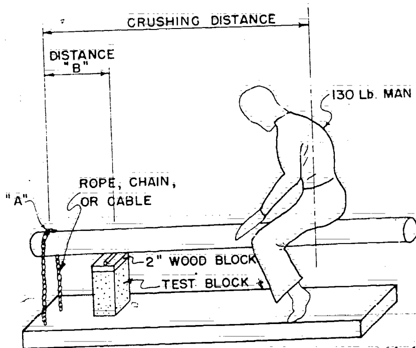
Figure 15. Simple lever test for determining strength of blocks (see Table 2).
