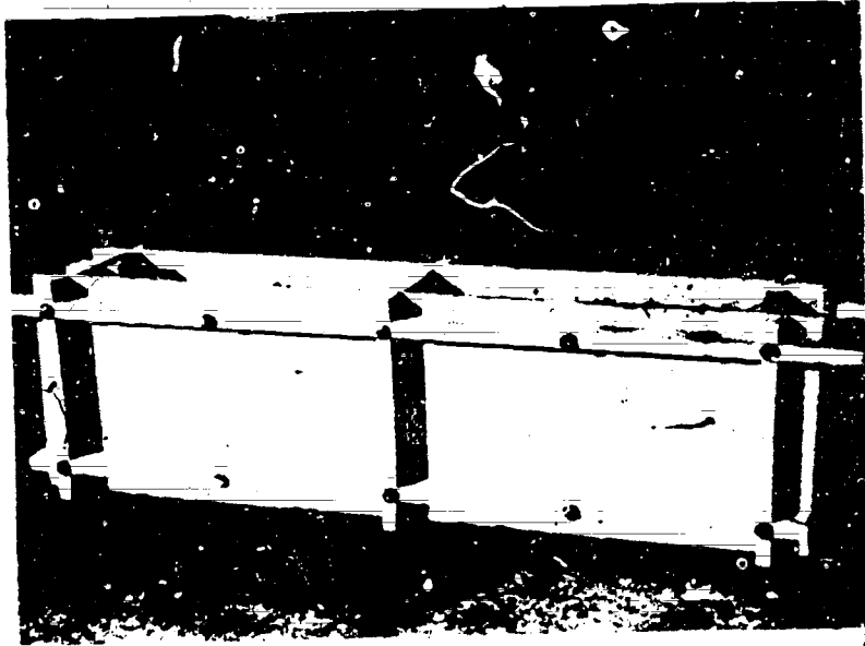
Figure 73. Straight form for rammed earth walls.
