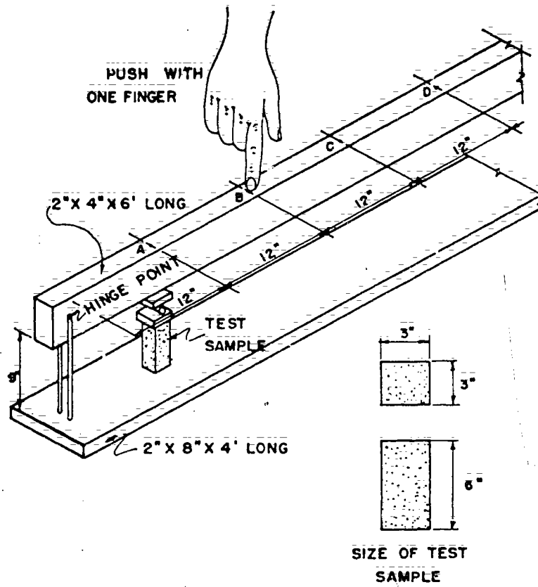
Figure 94. Simple lever tester for soils.
