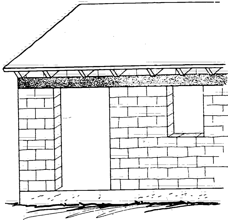
Figure 70. This shows a combination bond beam and lintel, made from reinforced concrete, that can be used, on low-ceiling houses.
