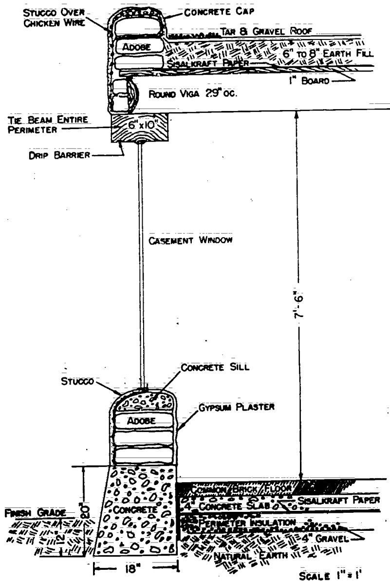
Figure 65. This typical wall section for adobe is used by a well known Albuquerque, N. M., adobe building contractor.
