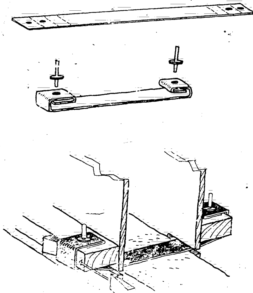
Figure 75. Thin metal strips such as these can be used instead of bolts to tie rammed earth forms together.
