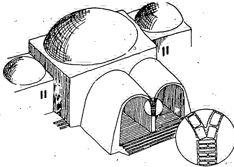
Figure 88. This style of earth dome and vault construction was used in a reconstruction program at New Gournia, Egypt.
