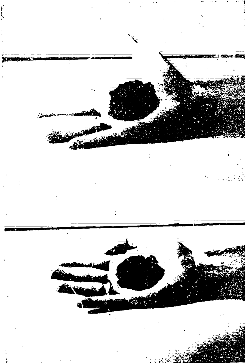
Figure 8c. A soil that did not react to the shaking test.
