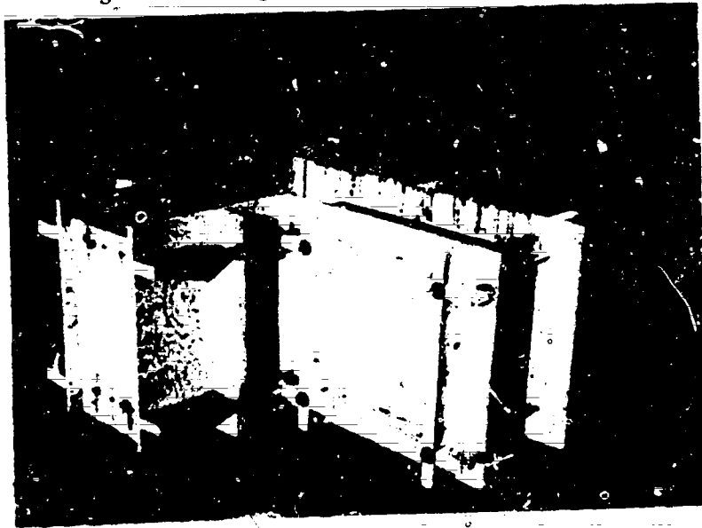
Figure 74. Plywood corner form for rammed earth walls.
