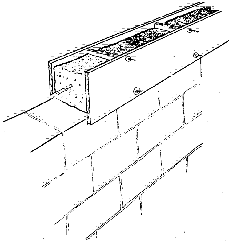
Figure 71: Forms like this can be used to pour concrete bond beams and lintels in place in the wall.
