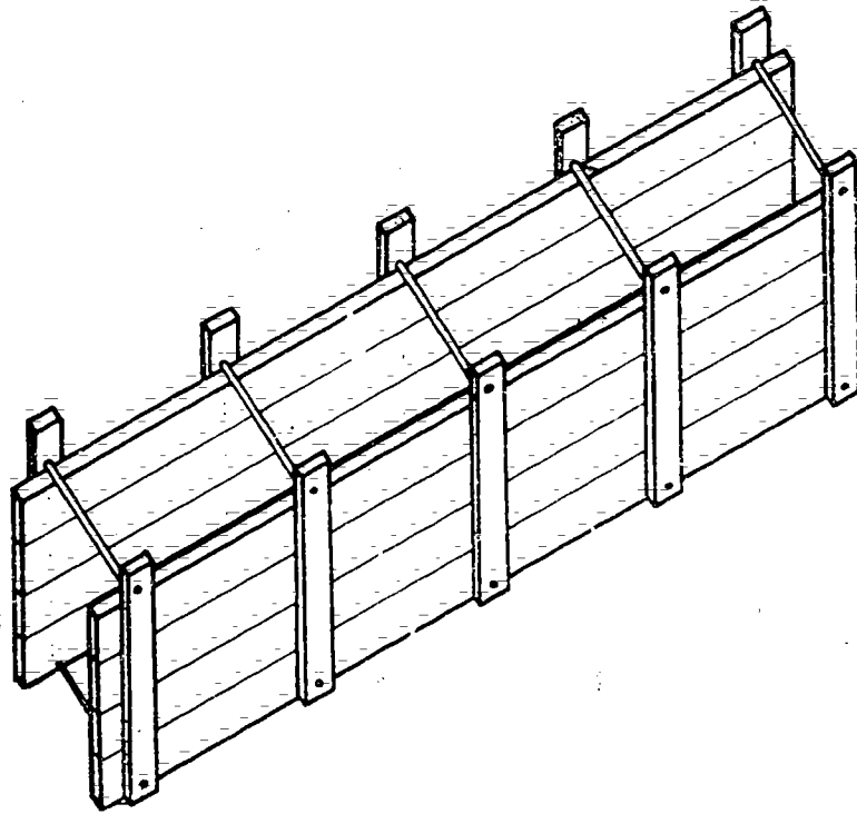
Figure 72. Form for ramming.
