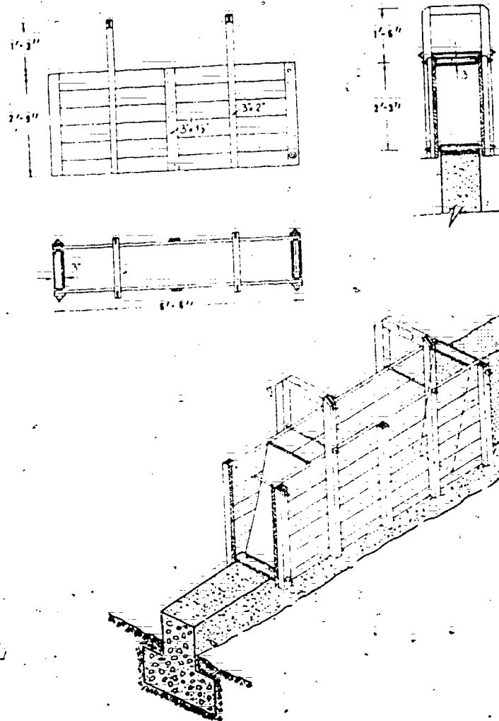
Figure 77. Form for ramming.
