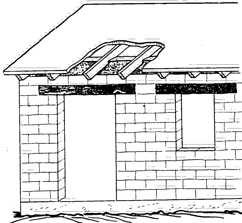
Figure 68. This shows how timber lintels are used above doors and windows. Above the lintels (in the cut-out section) is shown a concrete bond beam.
