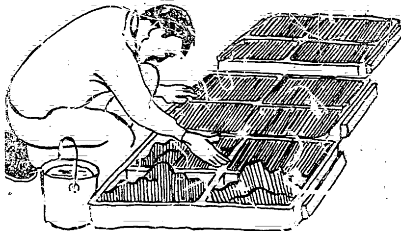
Figure 40. Kneading and leveling the blocks.
