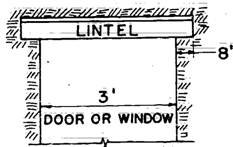
Figure 95. Wood lintel.
