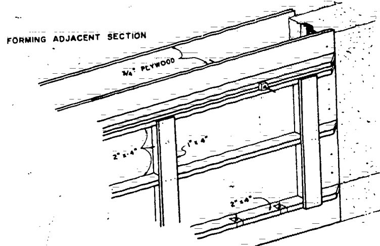
Figure 76. This is a special form that was designed to use the metal tie strips shown in Figure 75.
