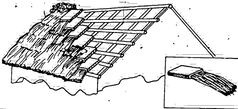
Figure 89. A thatched-earth tile roof of this design proved successful in research studies in India.
