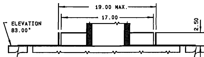
SEC. A-A FRONT VIEW, SUPPORT BRIDGE
